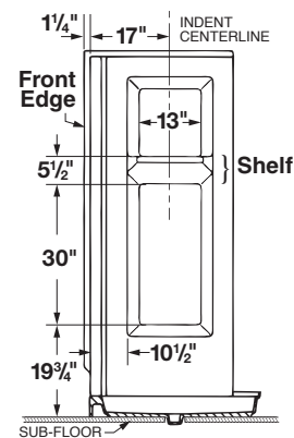
Valve Placement Dimensions
